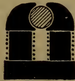
Diagram of magnetic circuit of T. H. bipolar dynamo. Leakage coefficient 1.3.
